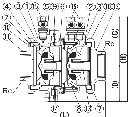
SCREWED END JIS (BSP) 20mm to 50mm
